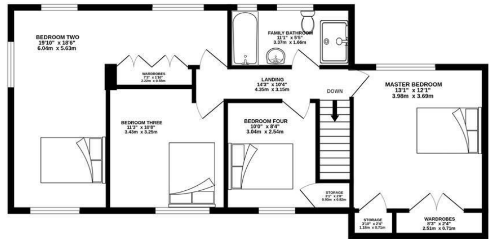
1ST FLOOR 755 sq.ft. (70.1 sq.m.) approx.
